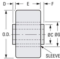
Fig. 1 With Chamfer
