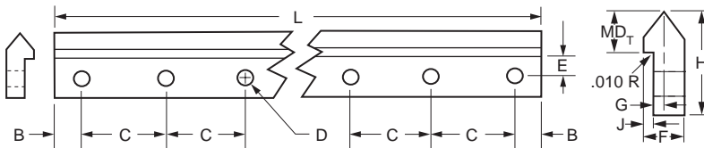
Standard Drilled Track Hole Spacing and Size
