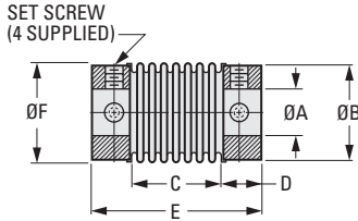
Fig. 1 Set Screw Type
